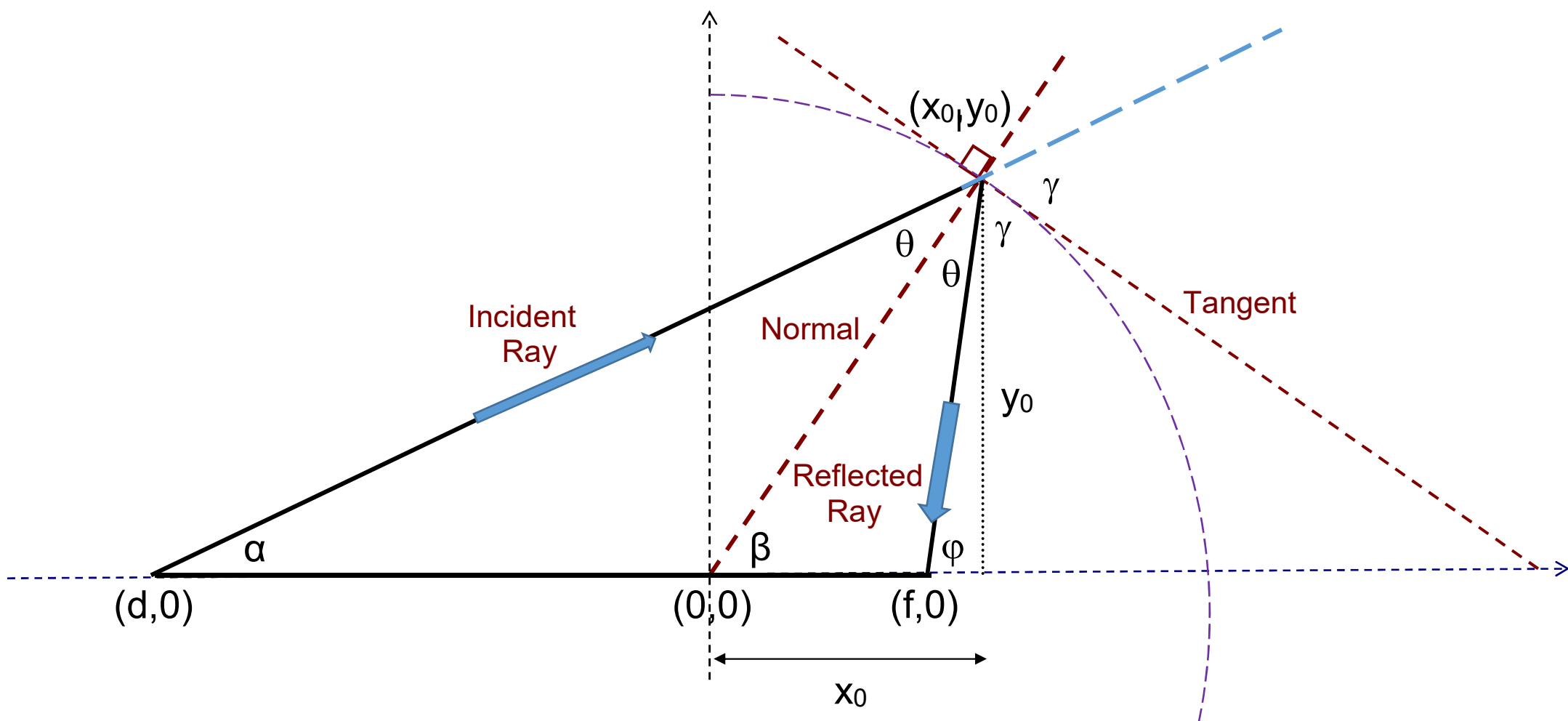
Figure 2.1: Interior bisector, exterior angle 2\gamma > 90^\circ
