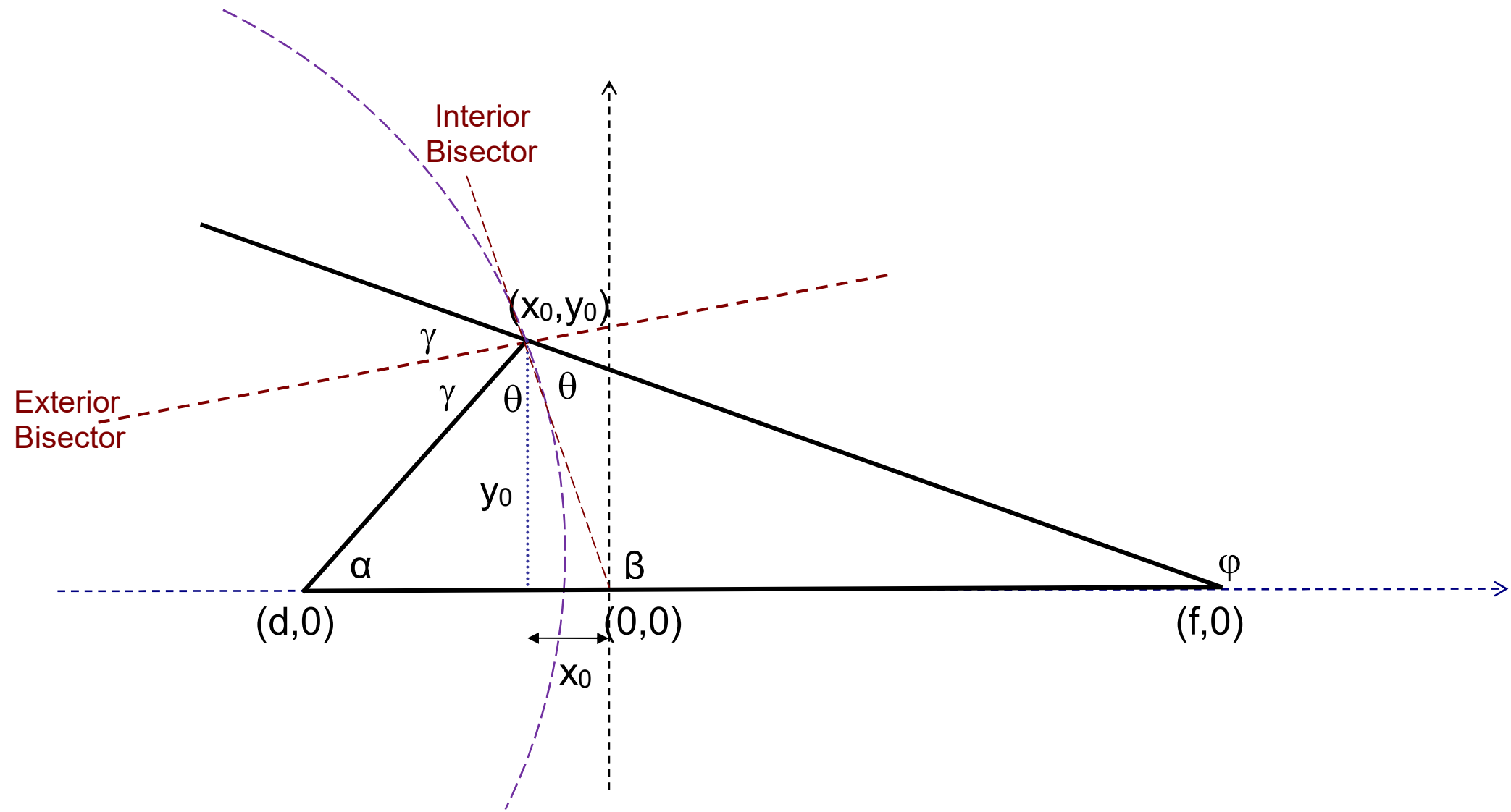
Figure 1: Exterior angle 2\gamma < 90^\circ
