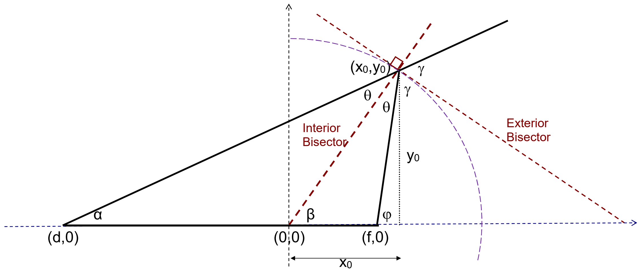
Figure 2: Exterior angle 2\gamma > 90^\circ
